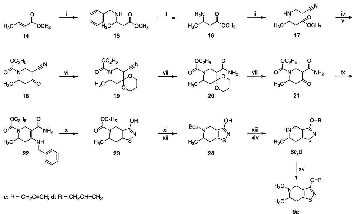
Scheme 2. Reagents and conditions: (i) C 6 H 5 CH 2 NH 2 , C 2 H 5 OH; (ii) NH 4 -HCOO, Pd-C (5%); (iii) CH 2 =CHCN, CH 3 OH; (iv) KOC(CH 3 ) 3 , toluene; (v) ClCOOC 2 H 5 , K 2 CO 3 ; (vi) HOCH 2 CH 2 CH 2 OH, TsOH, toluene, reflux; (vii) H 2 O 2 , NaOH, C 2 H 5 OH; (viii) HCl, H 2 O, THF; (ix) C 6 H 5 CH 2 NH 2 , toluene, reflux; (x) H 2 S, DMF, Br 2 ; (xi) HBr/AcOH (33%); (xii) (Boc) 2 O, K 2 CO 3 ; (xiii) CH≡CCH 2 Br, K 2 CO 3 , (C 4 H 9 ) 4 N-HSO 4 (c), CH 2 =CHCH 2 Br, K 2 CO 3 (d); (xiv) HCl, ether; (xv) HCOOH, CH 2 O, reflux.
