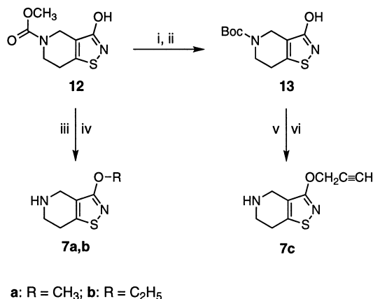
Scheme 1. Reagents and conditions: (i) HBr/AcOH (33%); (ii) (Boc) 2 O, K 2 CO 3 , K 2 CO 3 (1%)/CH 3 OH; (iii) CH 2 N 2 ( a ), (C 2 H 5 ) 2 SO 4 , (C 4 H 9 ) 4 N·HSO 4 , NaOH ( b ); (iv) KOH/CH 3 OH; (v) CH≡CCH 2 Br, K 2 CO 3 , (C 4 H 9 ) 4 N·HSO 4 ; (vi) HCl, ether, NaOH.
